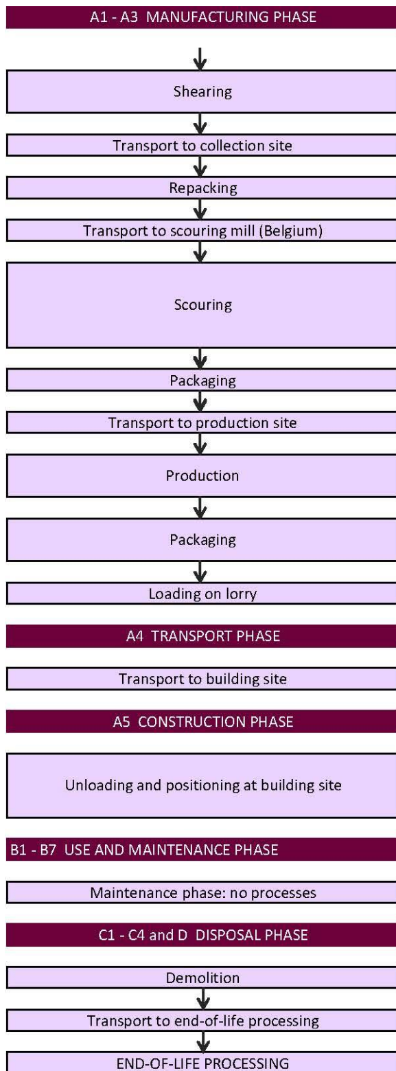
Figure 2: Flowchart Isolena sheepwool insulation with Ionic Protect®
